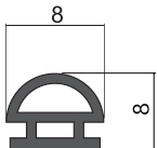
10MM PVC for single glass
