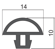
cushion PVC for door frame
