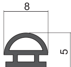
6MM PVC for double glass
